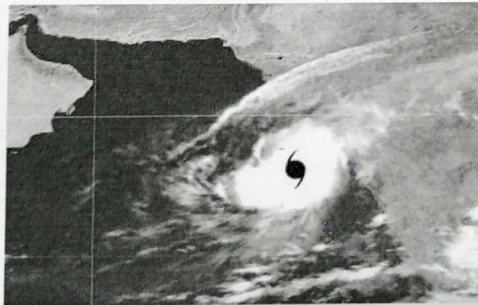
IR Satellite imagery at 1000 PST on 26 October 2019
